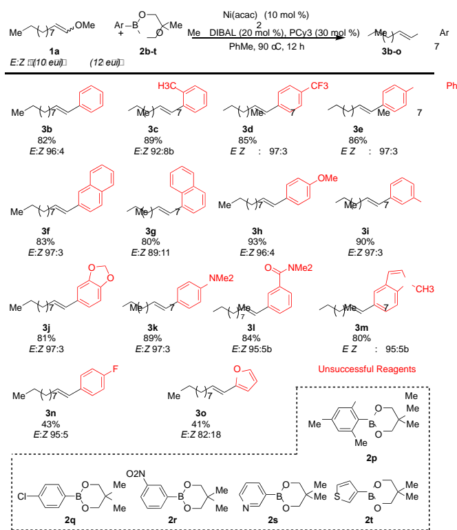
Scheme 2. Cross-coupling of alkenyl ether 1a with different boronic esters
