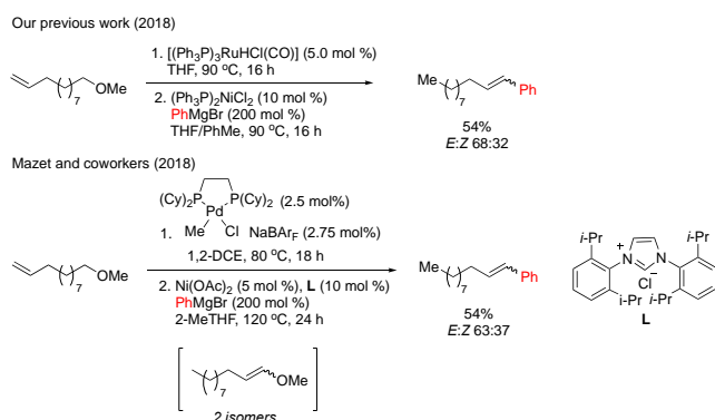
Figure 1. Previously reported tandem metal-catalyzed 'chain-walking'/nickel-catalyzed Kumada cross-coupling
