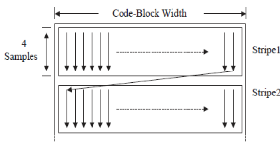
Fig.1 EBCOT Process
