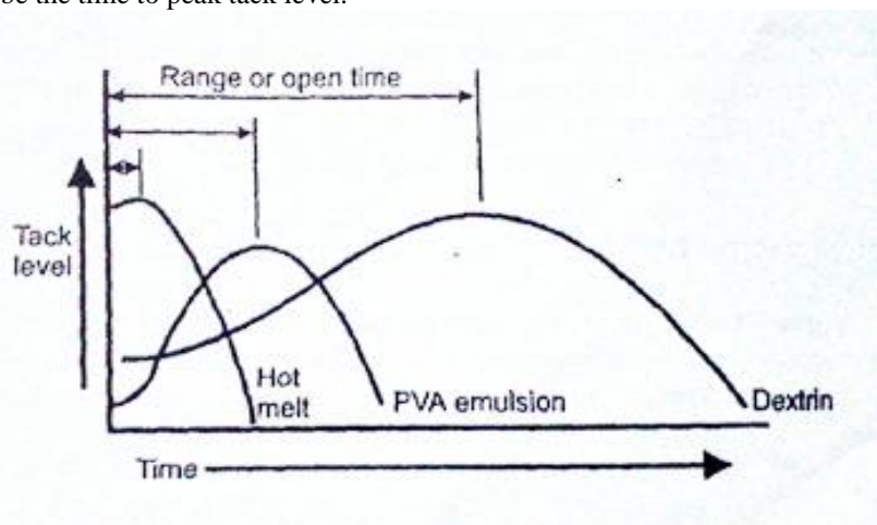
Fig.1. “Open time” or “tack & range” for three adhesive types.
